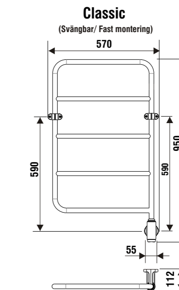
Oil-filled with electric heating cartridge 75W
